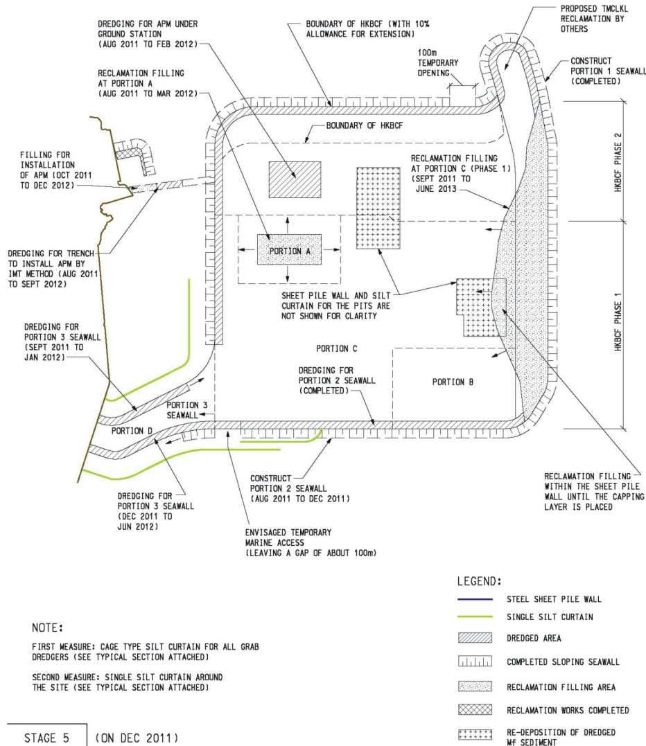
Figure 4 - Construction Sequence of HKBCF
